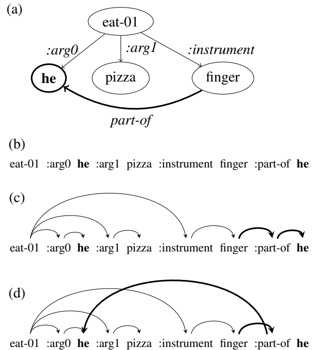
Figure 1: (a) AMR for the sentence He ate the pizza with his fingers and different input representations: (b) sequential; (c) tree-structured; (d) graph-structured. The nodes and edges in bold highlight a reentrancy.
